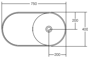
LUNE 750 BASIN 750 W x 400 D x 150 H
