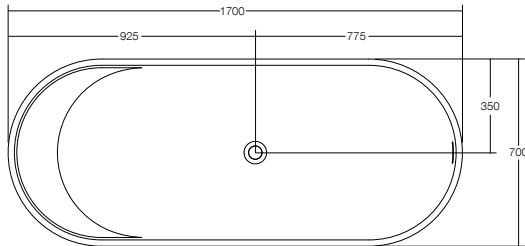
LUNE FREESTANDING BATH 1700 W x 700 D x 600 H
