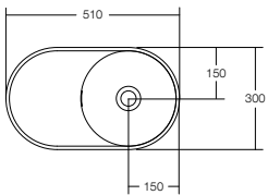
LUNE 510 BASIN 510 W x 300 D x 110 H
