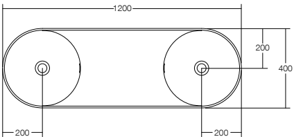
LUNE 1200 BASIN 1200 W x 400 D x 150 H
