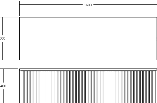
RITMO 1600 CABINET 1600 W x 500 D x 400 H
