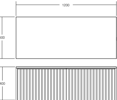
RITMO 1200 CABINET 1200 W x 500 D x 400 H
