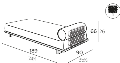
EMRSB189-K-S CU-EMRSB185 EMIR MODULE SUNBED 189
