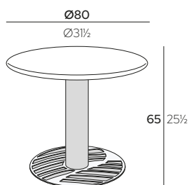
GHFD080-K-X-P GHAF LOUNGE TABLE Ø80 CM
